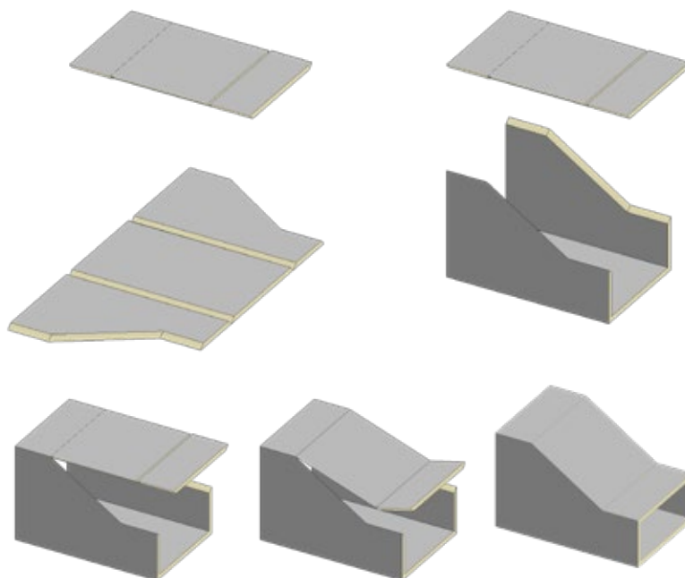
Boot take-off
