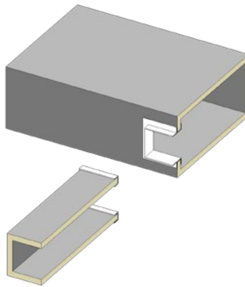
Flanged connection
